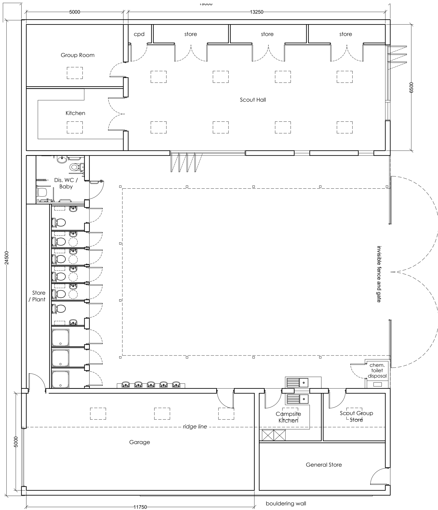
Floor Plan
