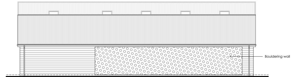
Garage South Facing Elevation Not to scale
